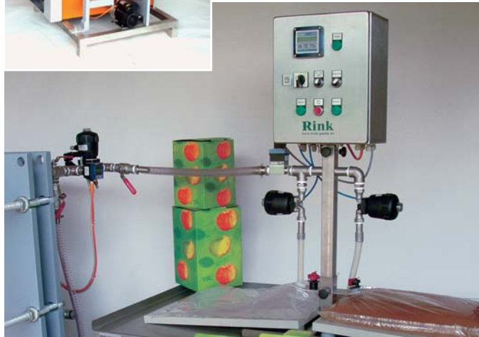
Bag in Box Dosierautomat DF 1000 2-stellig
